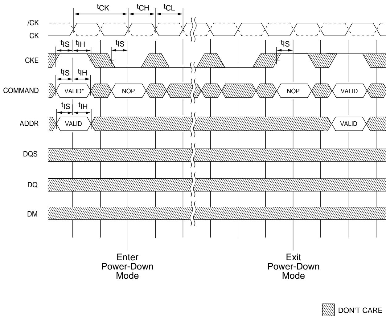
Figure 39 - POWER-DOWN MODE
